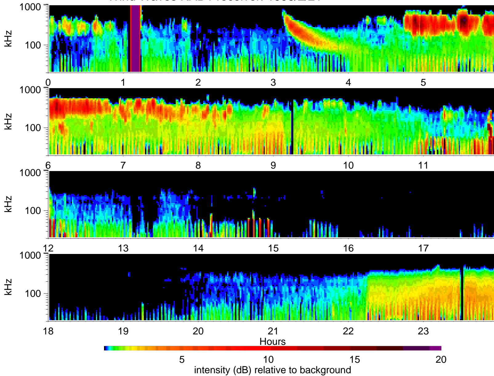
Wind Waves RAD1 receiver: 1996/2/21
