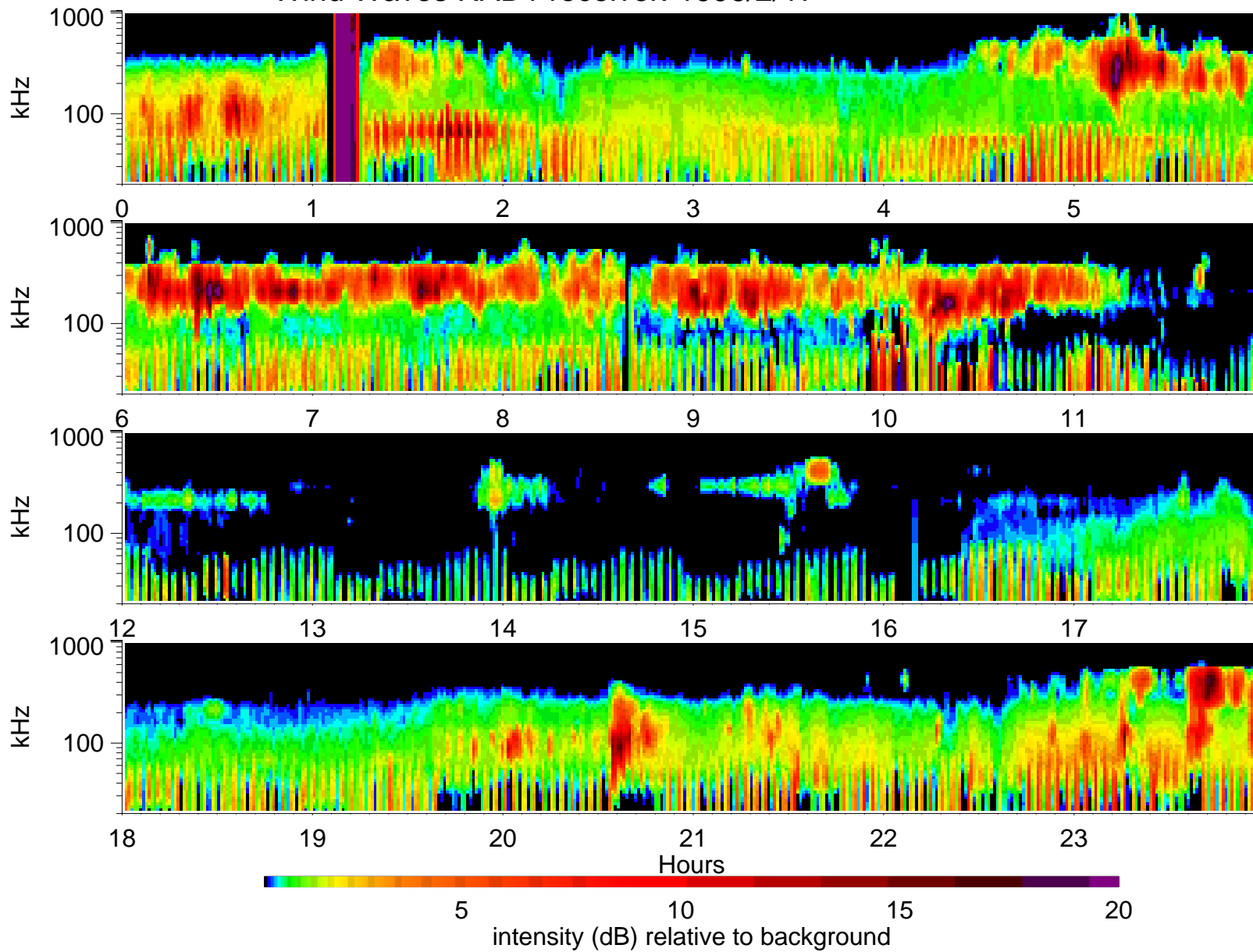
Wind Waves RAD1 receiver: 1996/2/17
