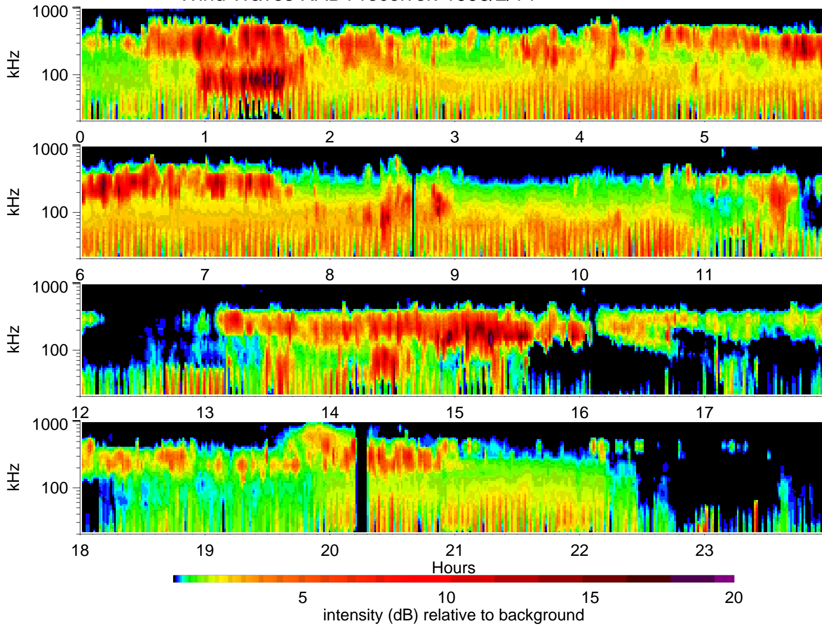
Wind Waves RAD1 receiver: 1996/2/14
