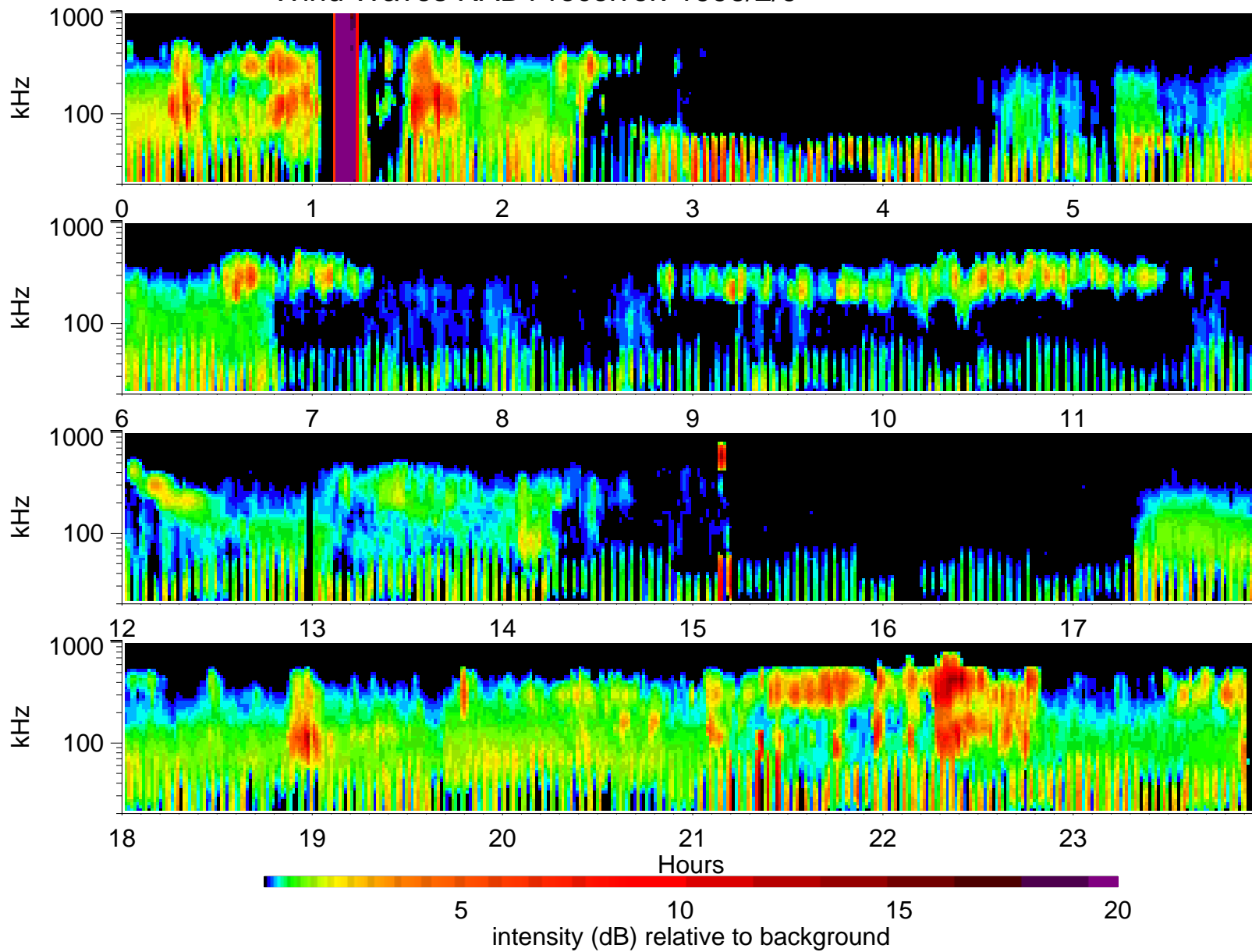
Wind Waves RAD1 receiver: 1996/2/9
