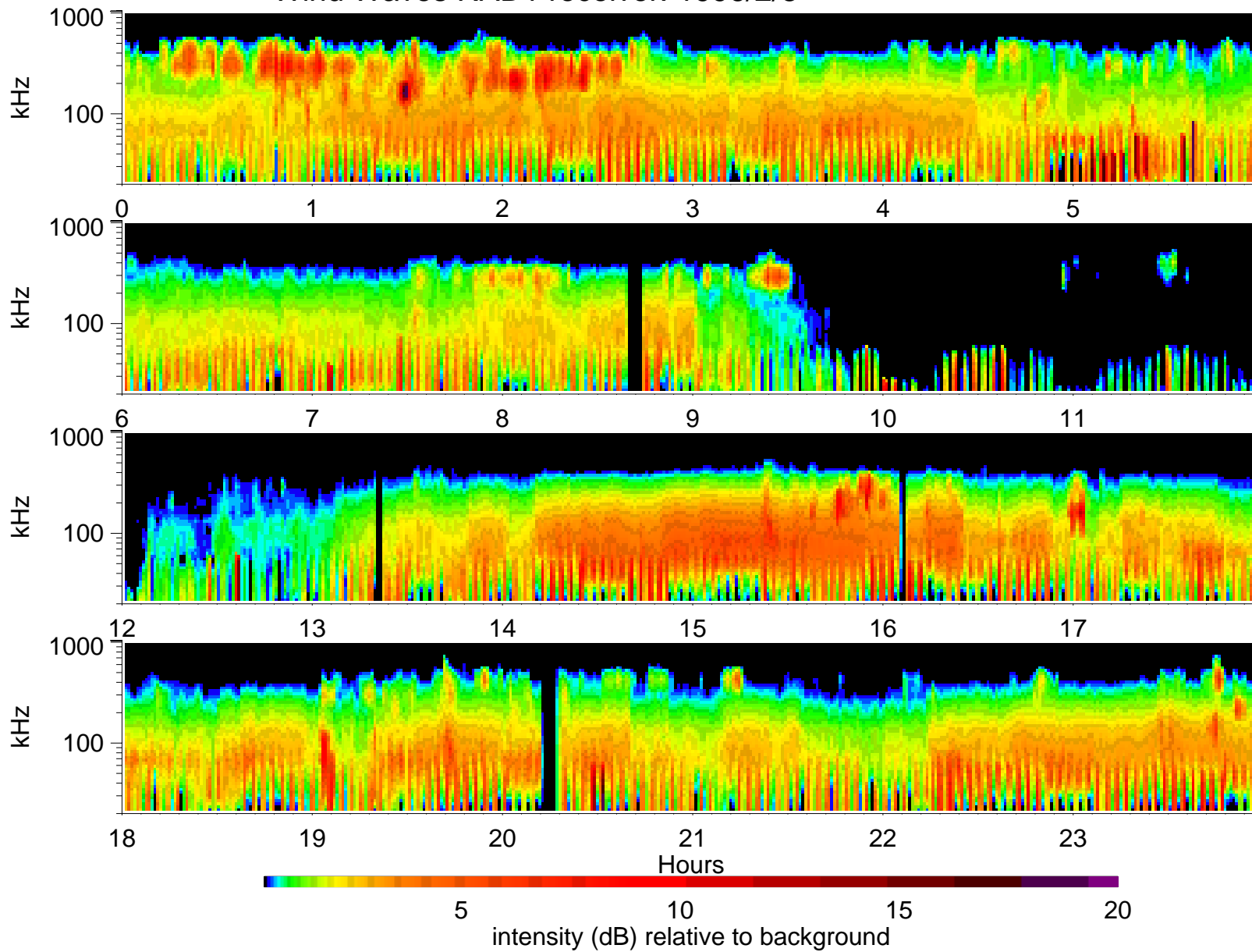
Wind Waves RAD1 receiver: 1996/2/8
