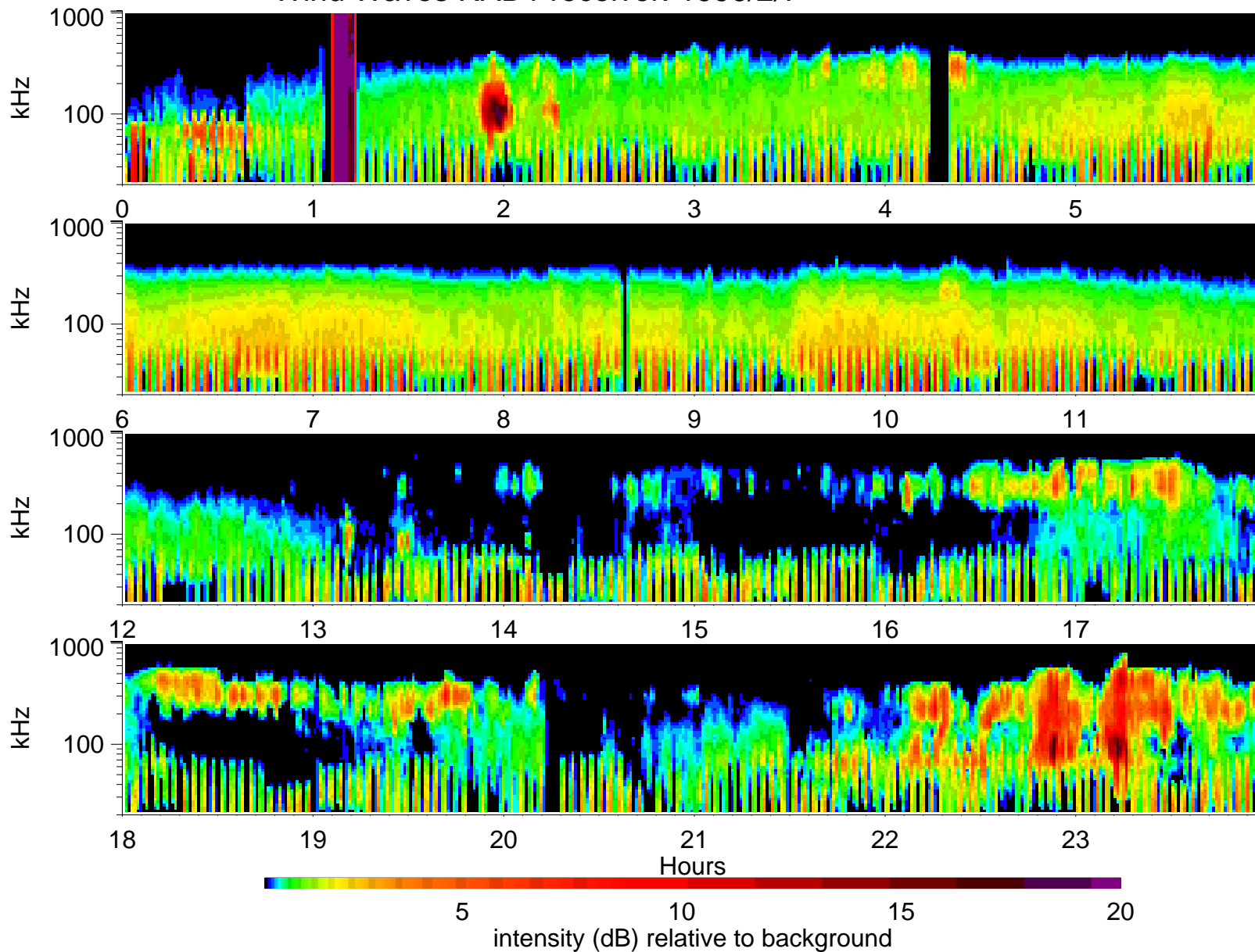
Wind Waves RAD1 receiver: 1996/2/7
