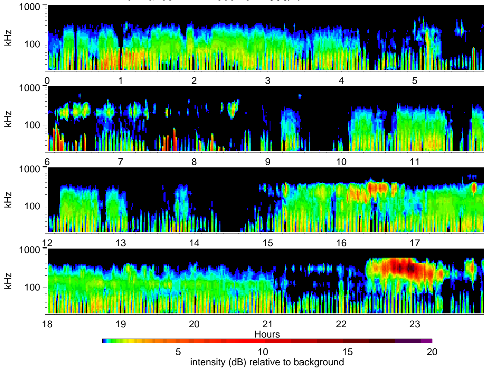
Wind Waves RAD1 receiver: 1996/2/4
