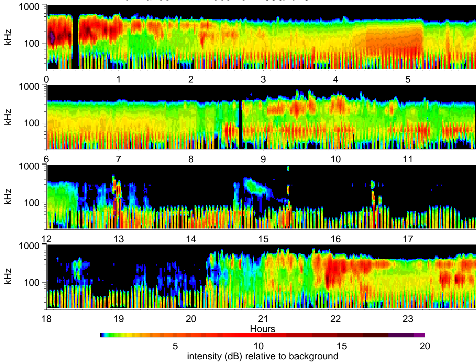
Wind Waves RAD1 receiver: 1996/1/25
