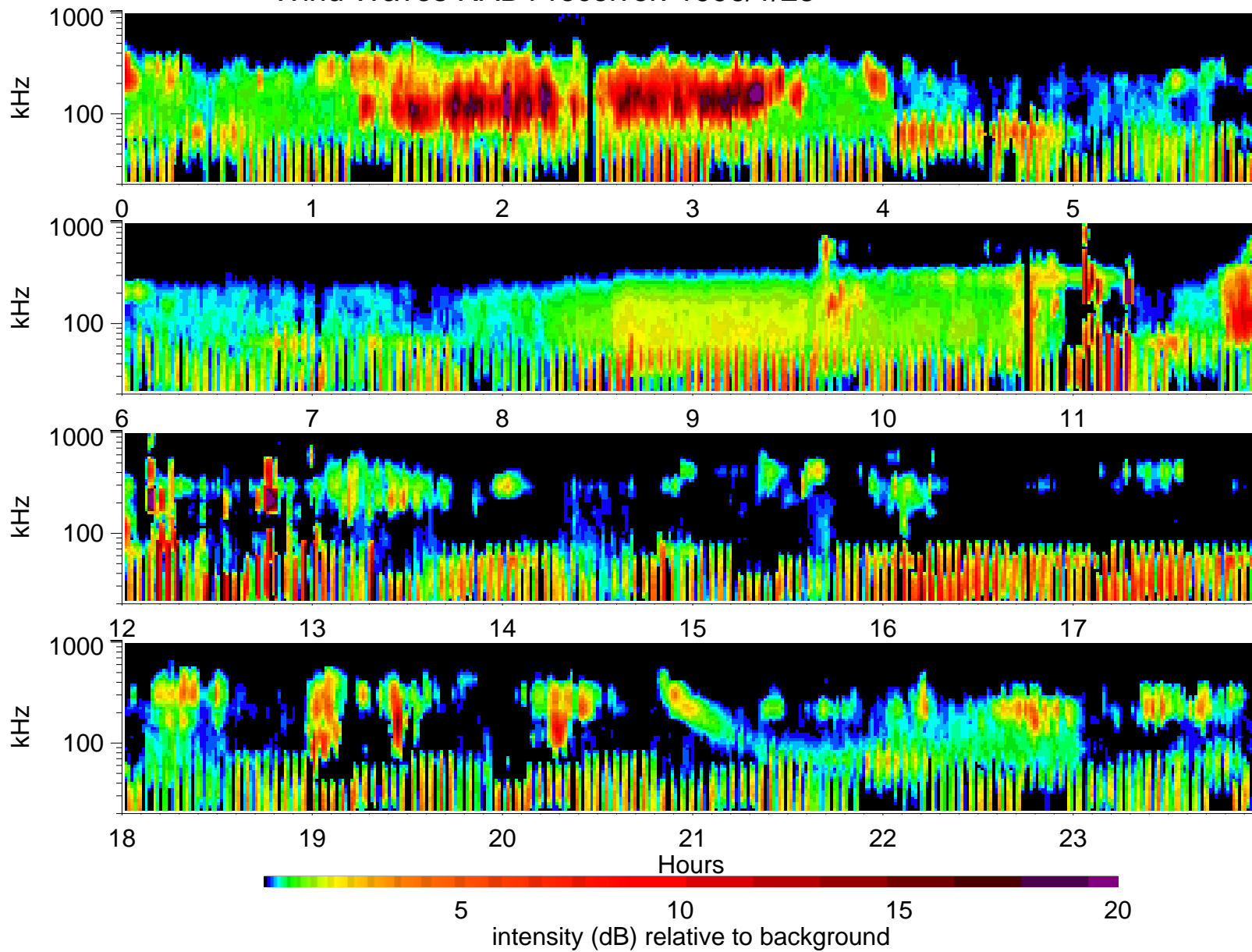
Wind Waves RAD1 receiver: 1996/1/23
