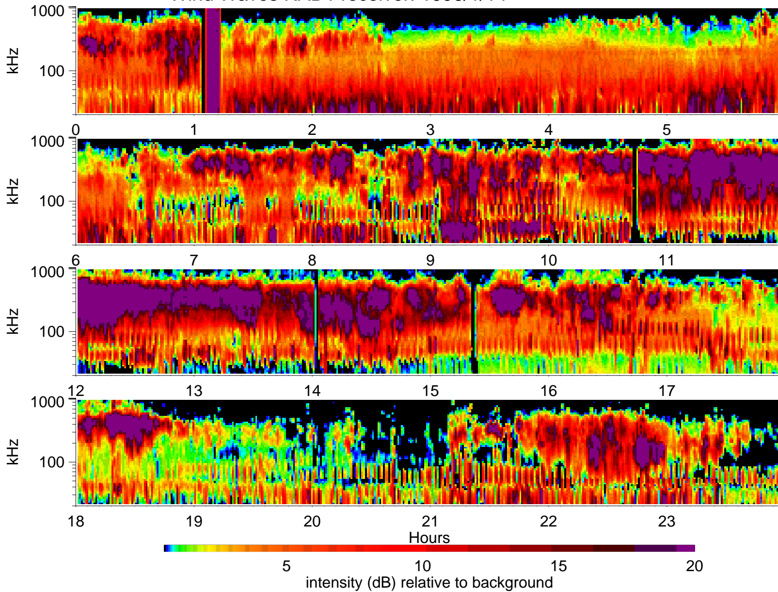
Wind Waves RAD1 receiver: 1996/1/14
