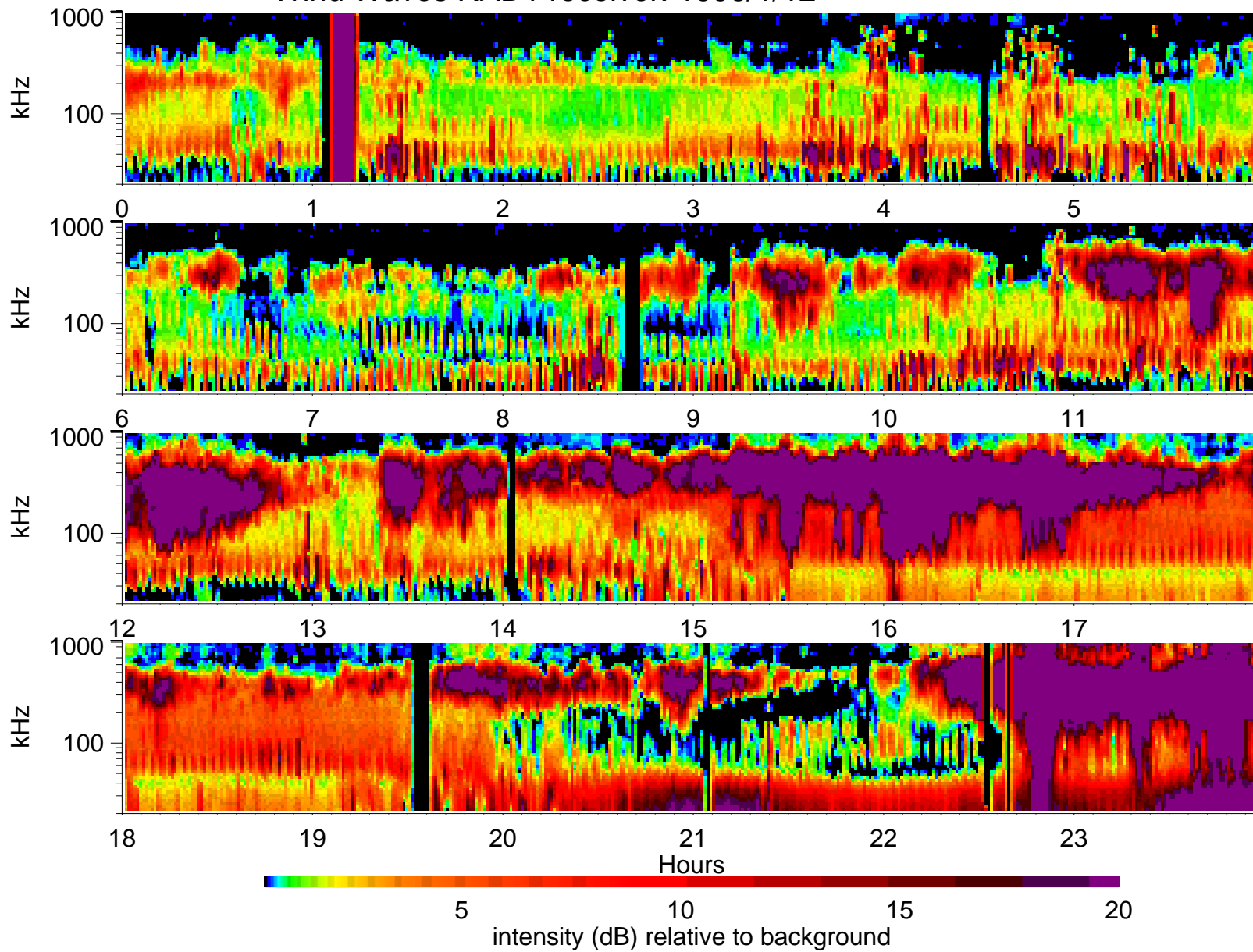
Wind Waves RAD1 receiver: 1996/1/12
