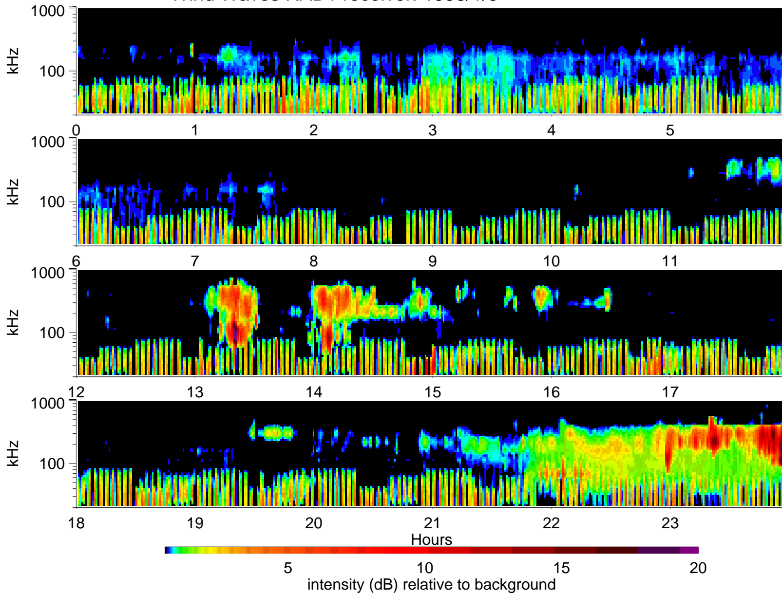
Wind Waves RAD1 receiver: 1996/1/9
