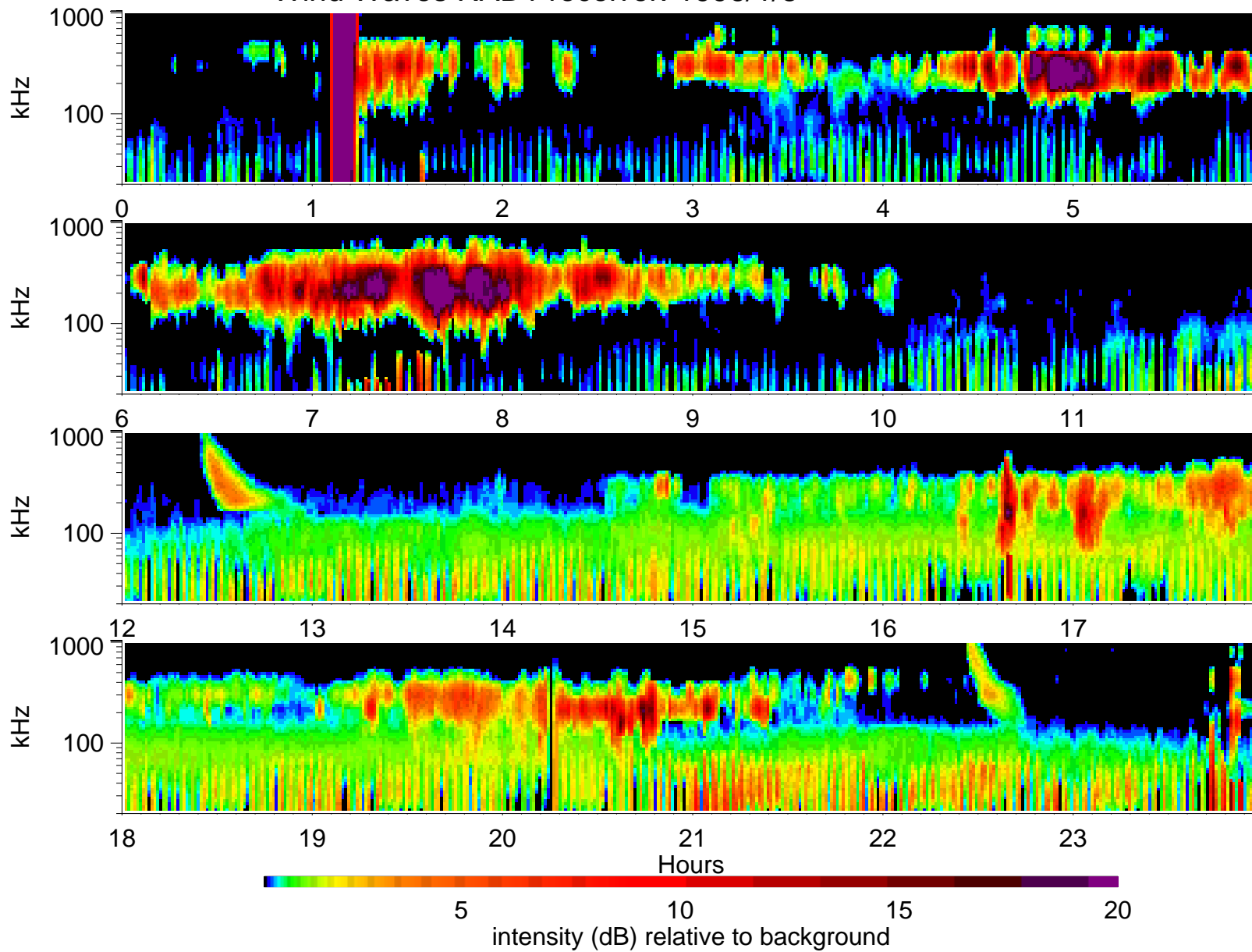
Wind Waves RAD1 receiver: 1996/1/8
