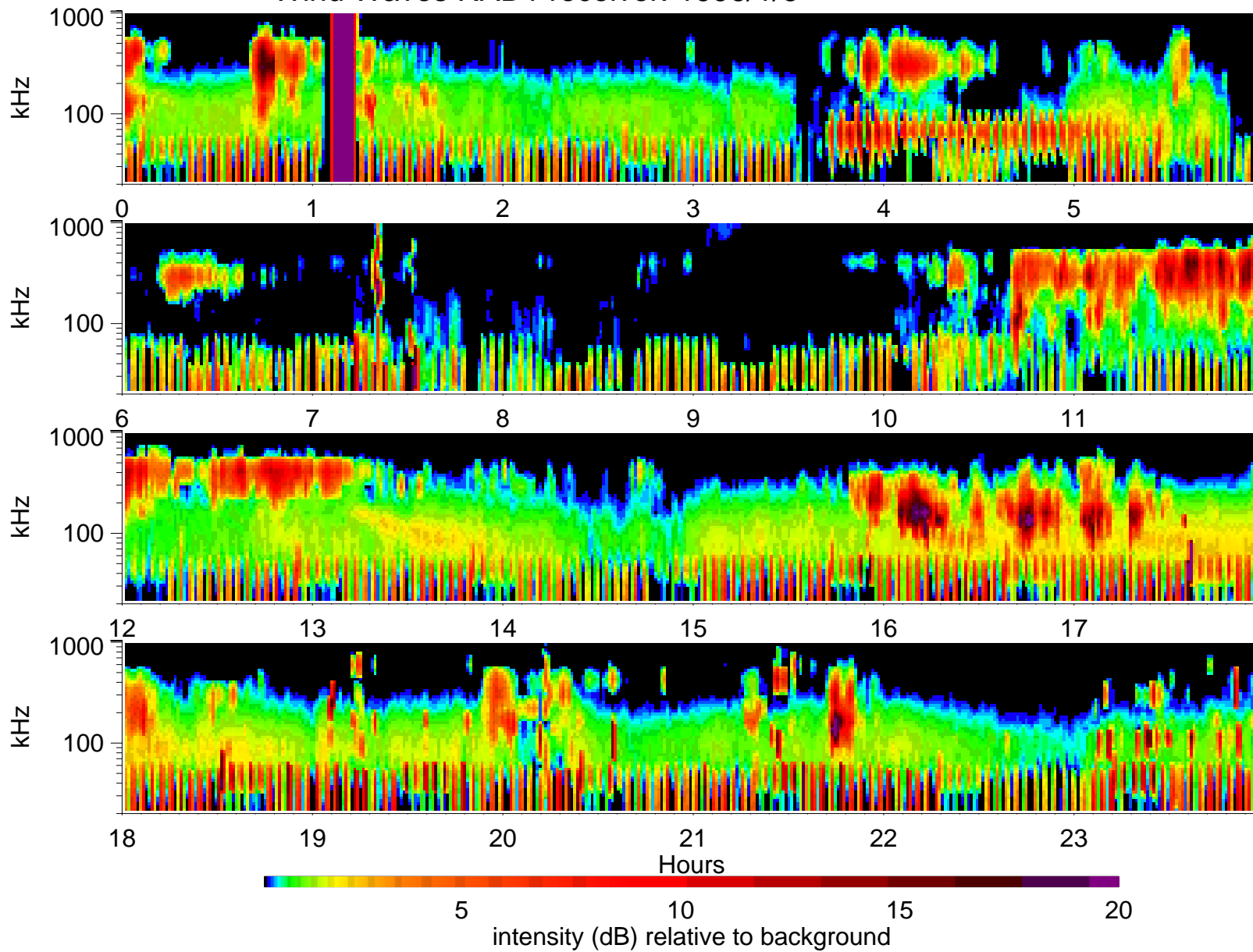
Wind Waves RAD1 receiver: 1996/1/6
