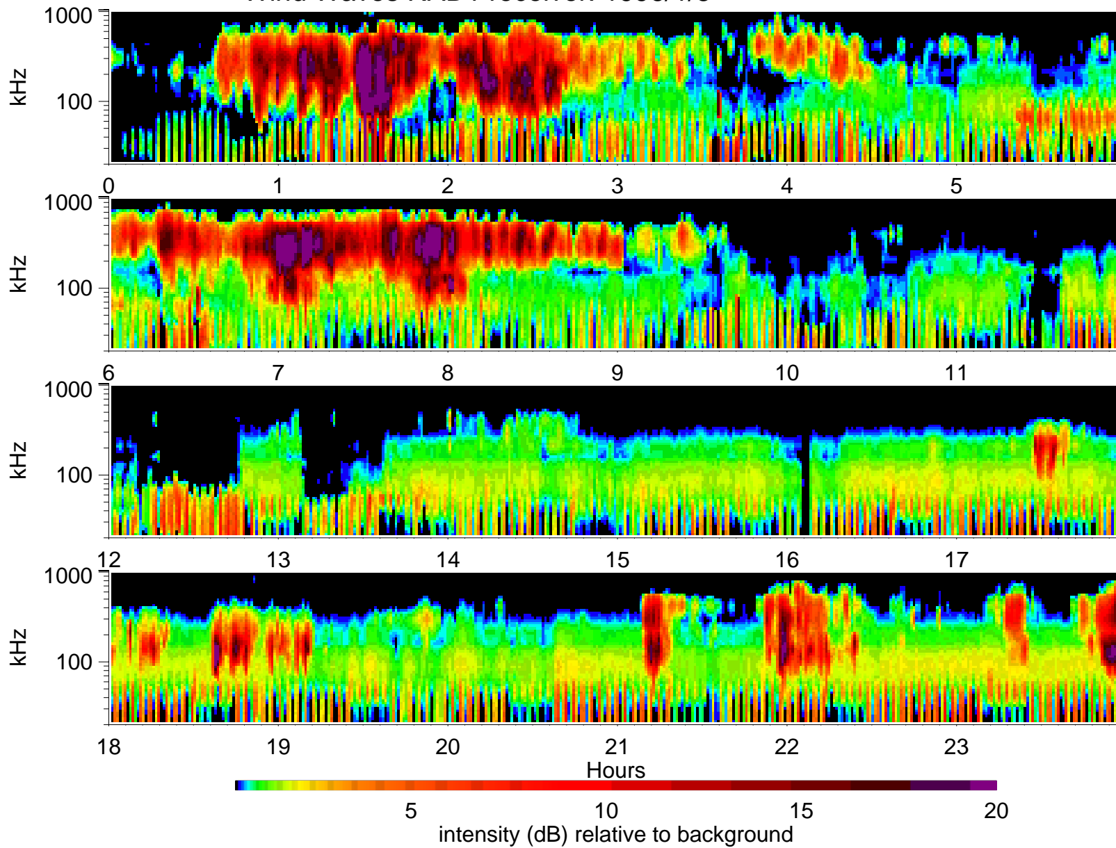
Wind Waves RAD1 receiver: 1996/1/5
