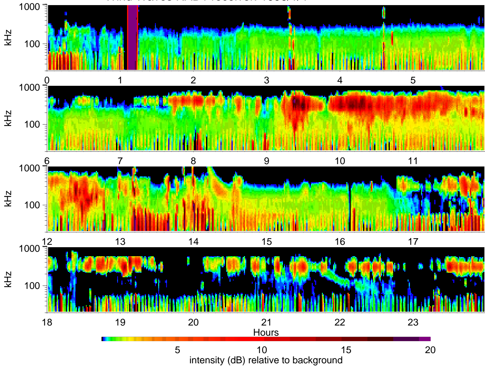
Wind Waves RAD1 receiver: 1996/1/4
