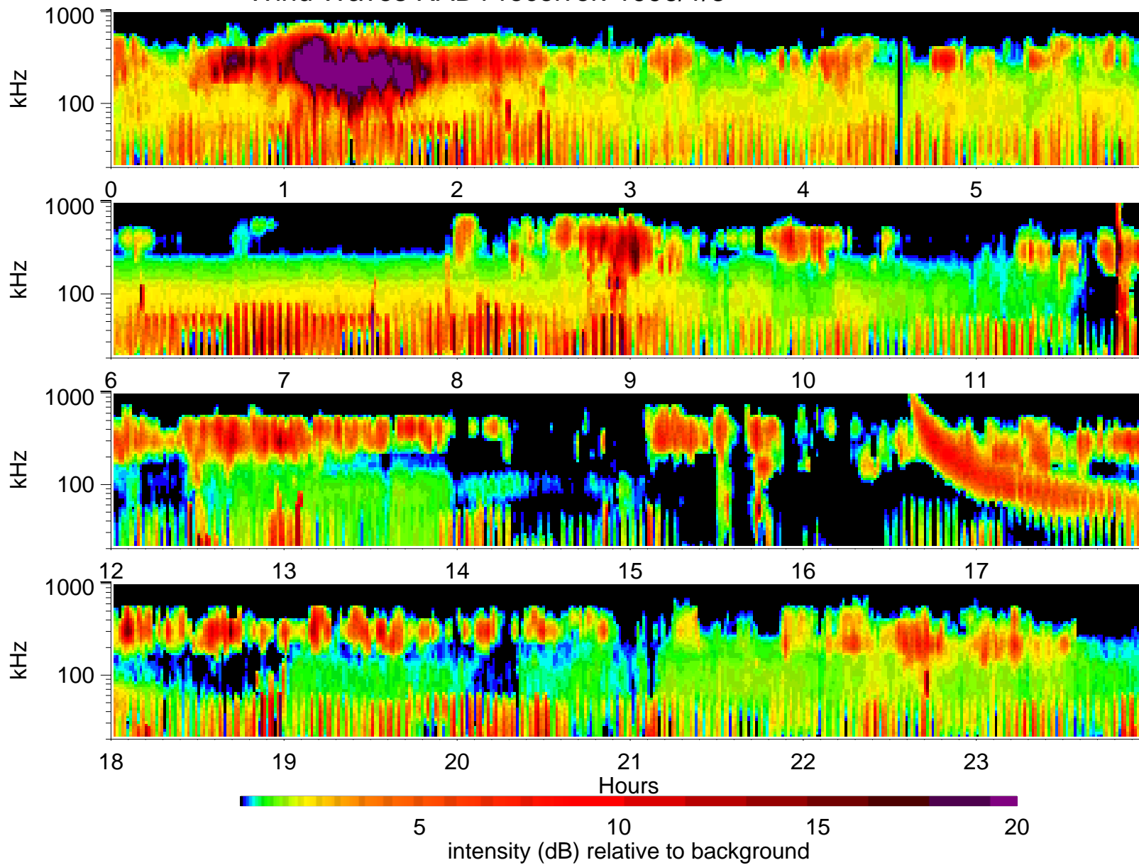
Wind Waves RAD1 receiver: 1996/1/3
