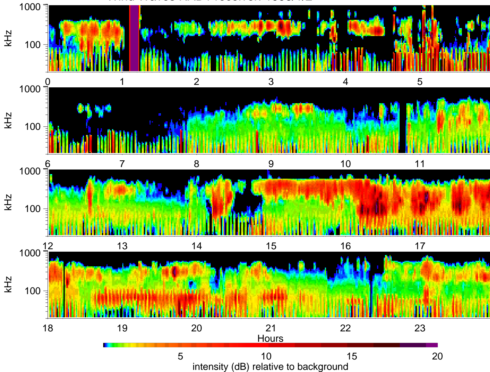
Wind Waves RAD1 receiver: 1996/1/2
