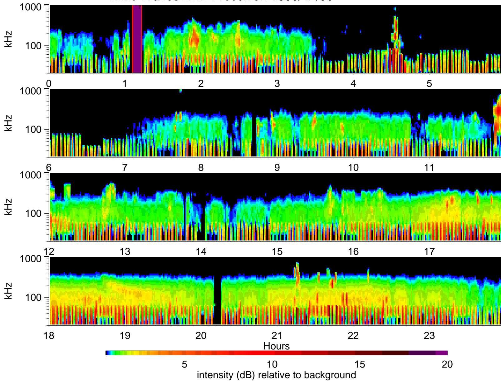
Wind Waves RAD1 receiver: 1995/12/30
