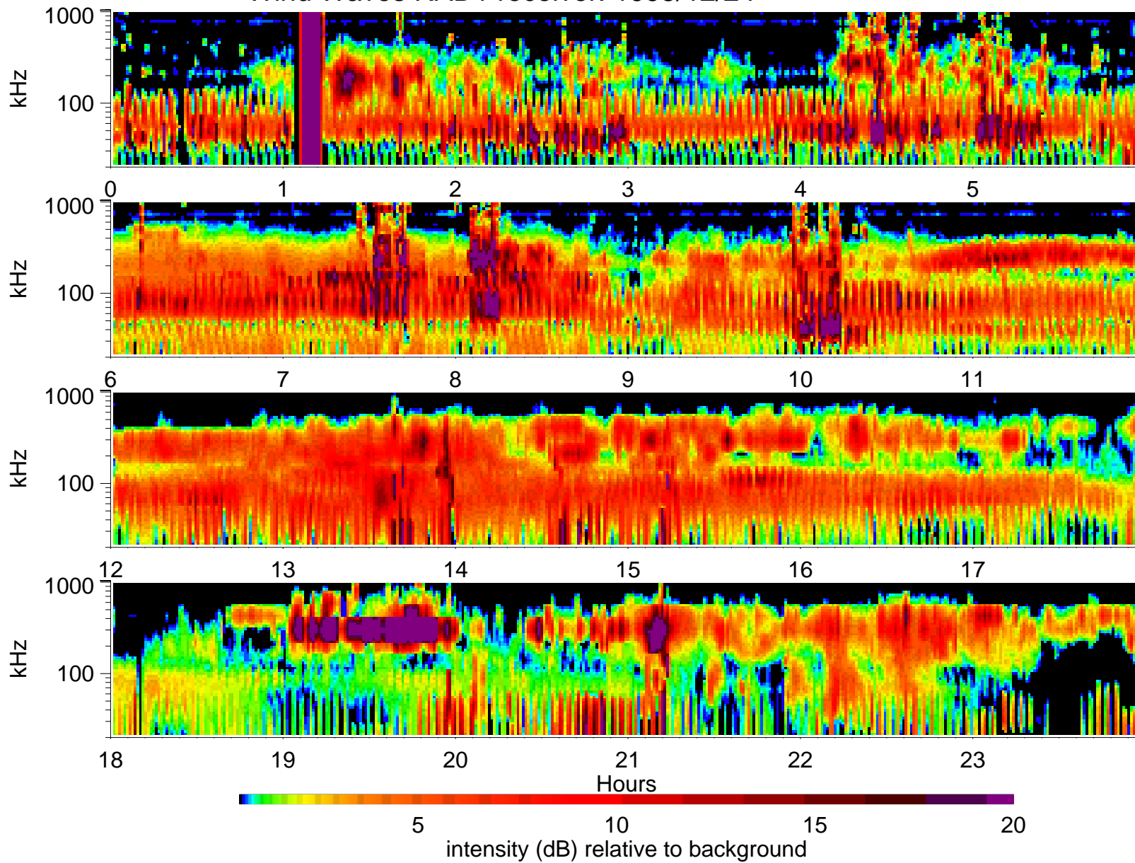
Wind Waves RAD1 receiver: 1995/12/24
