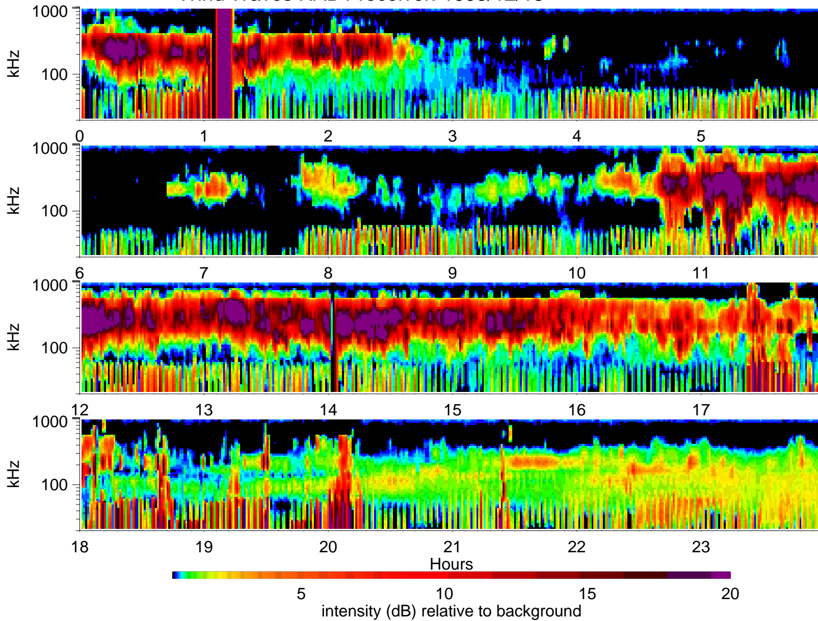
Wind Waves RAD1 receiver: 1995/12/18
