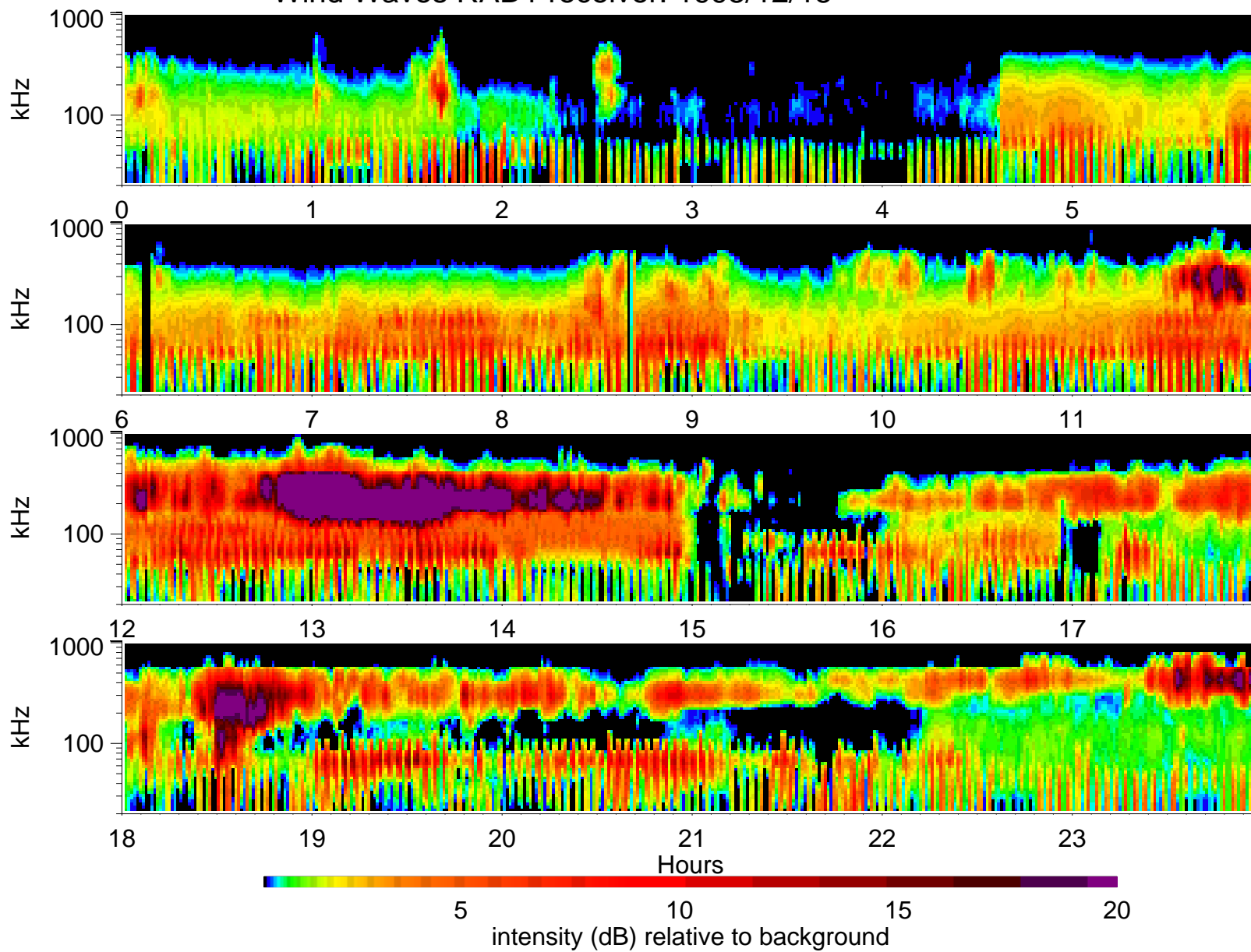
Wind Waves RAD1 receiver: 1995/12/15
