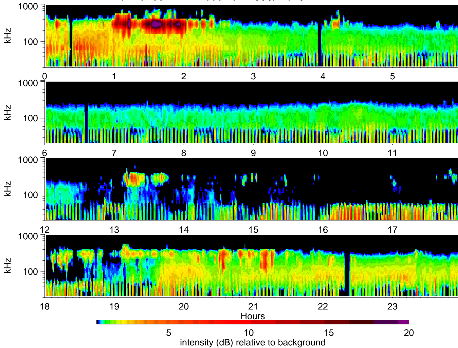
Wind Waves RAD1 receiver: 1995/12/13
