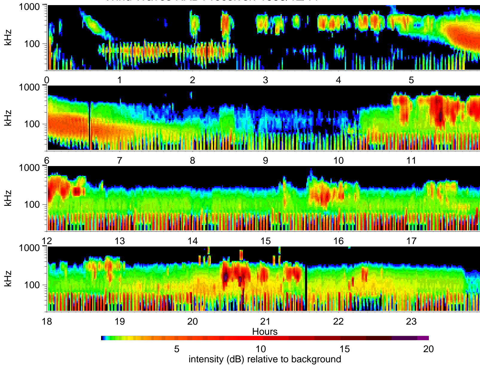
Wind Waves RAD1 receiver: 1995/12/11
