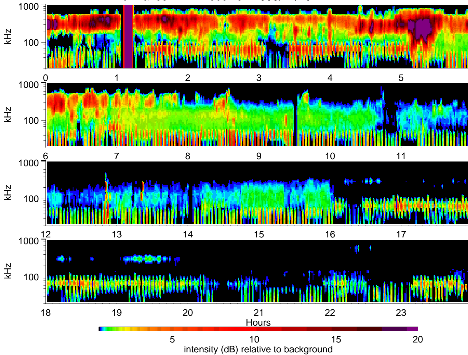
Wind Waves RAD1 receiver: 1995/12/10
