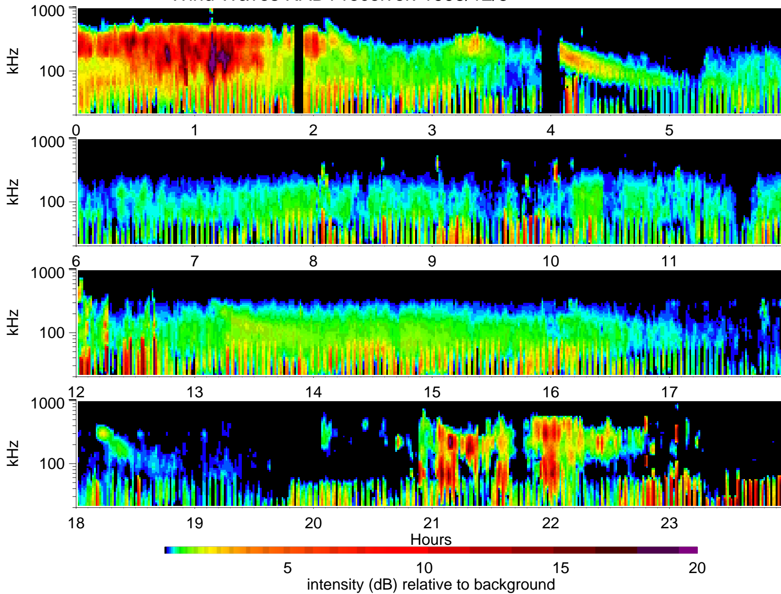
Wind Waves RAD1 receiver: 1995/12/5
