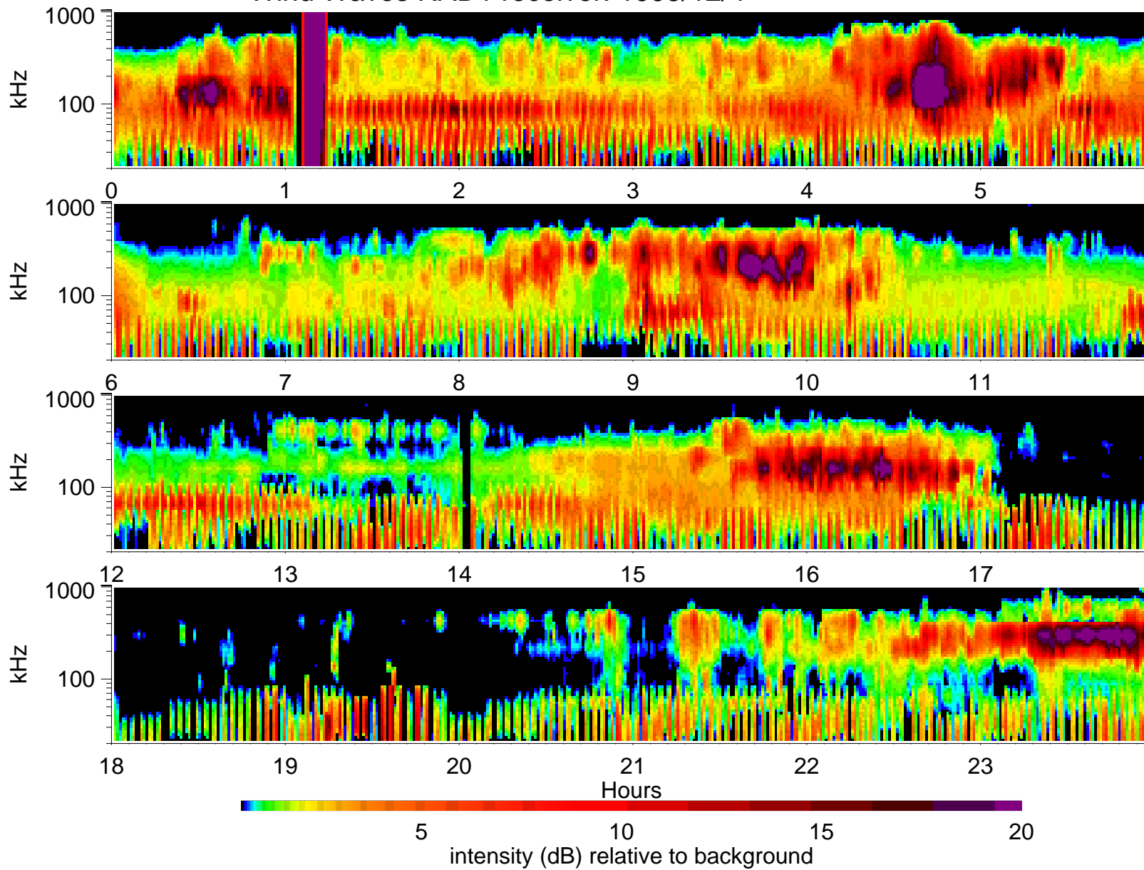
Wind Waves RAD1 receiver: 1995/12/4
