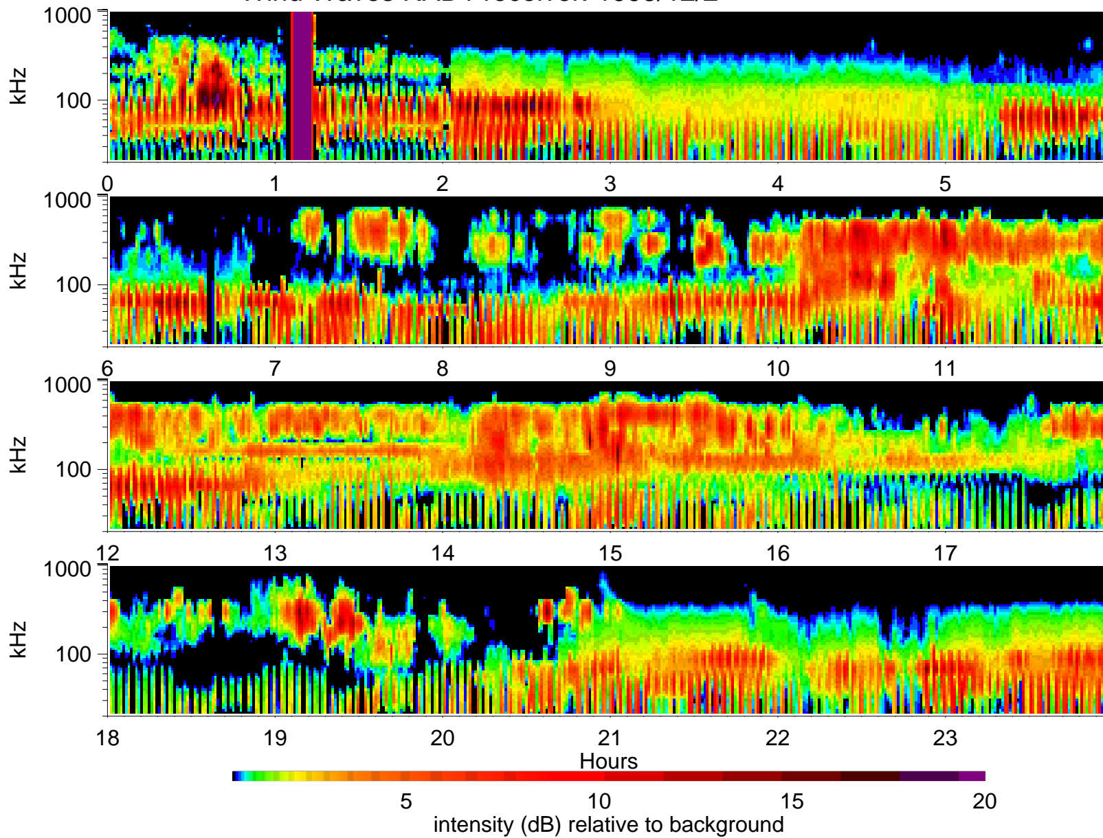
Wind Waves RAD1 receiver: 1995/12/2
