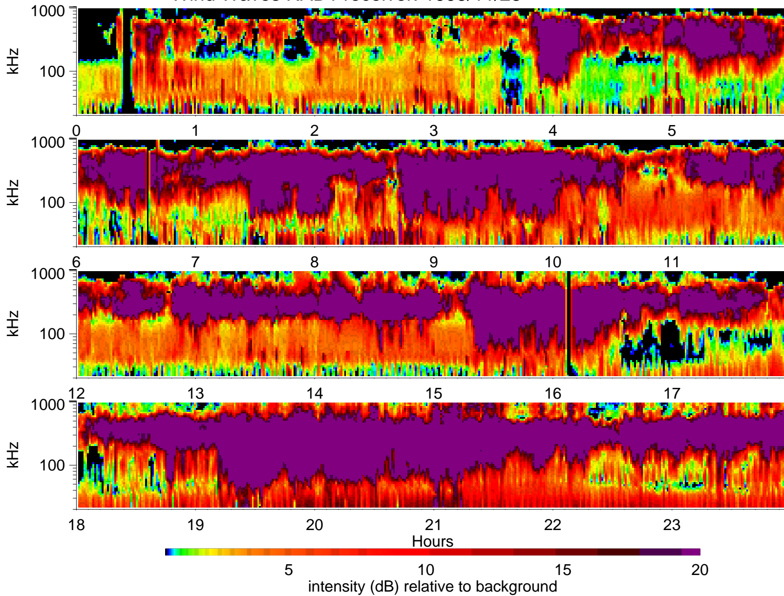
Wind Waves RAD1 receiver: 1995/11/28
