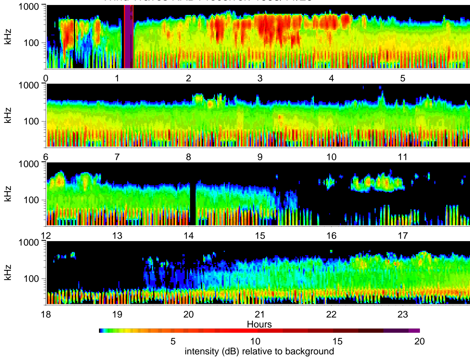
Wind Waves RAD1 receiver: 1995/11/26
