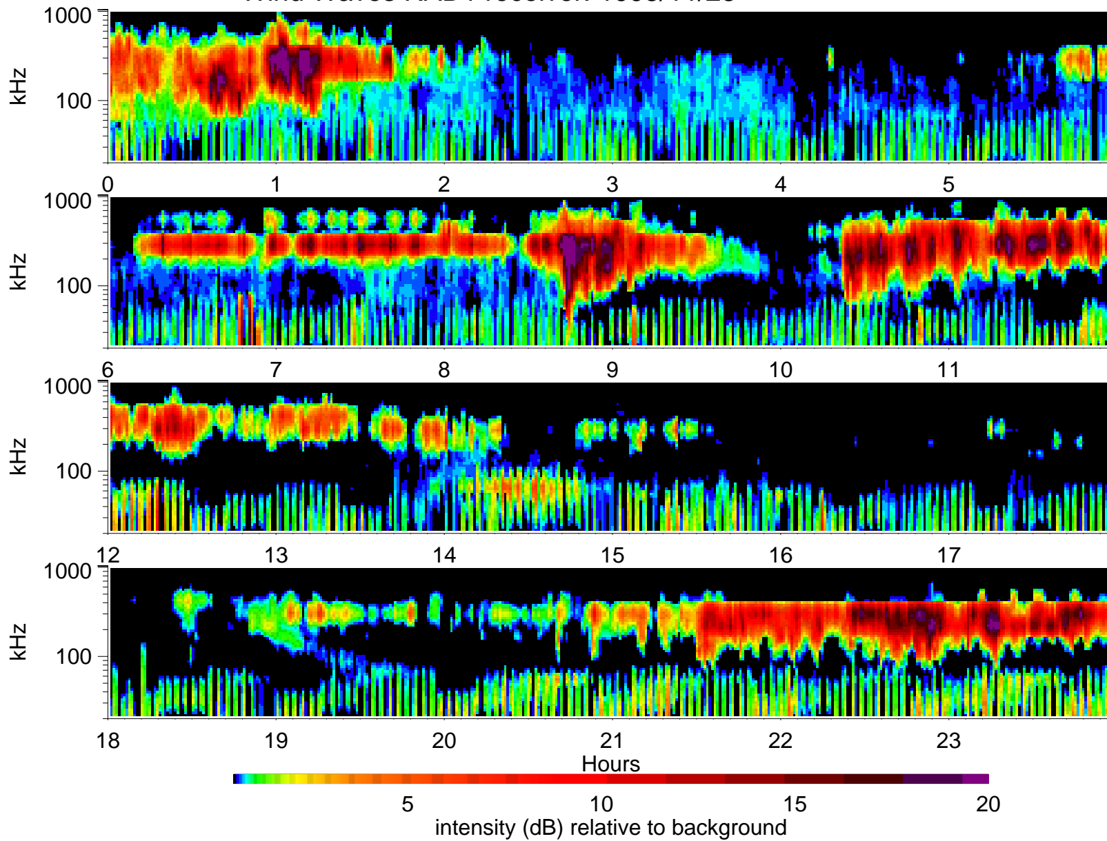
Wind Waves RAD1 receiver: 1995/11/23
