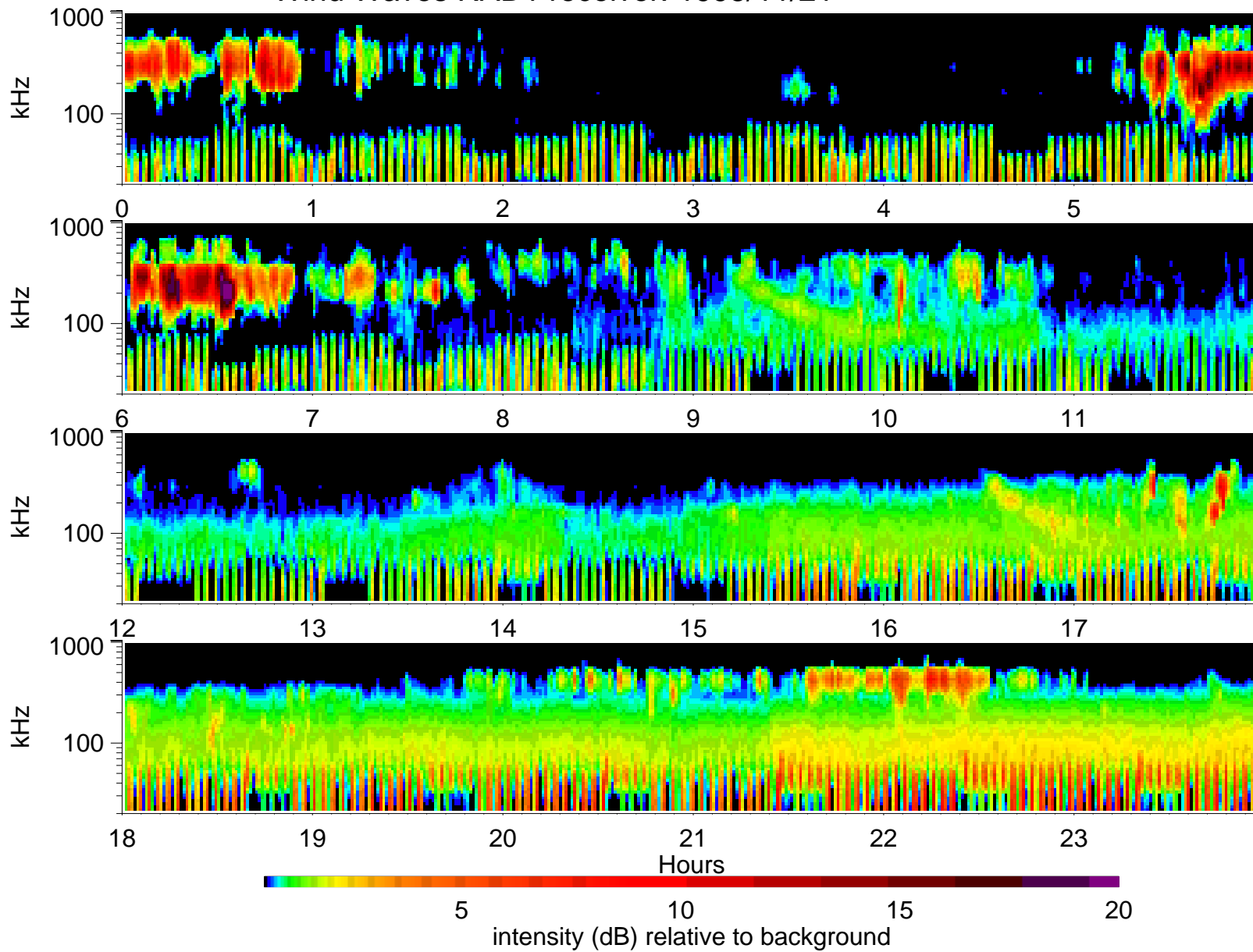
Wind Waves RAD1 receiver: 1995/11/21
