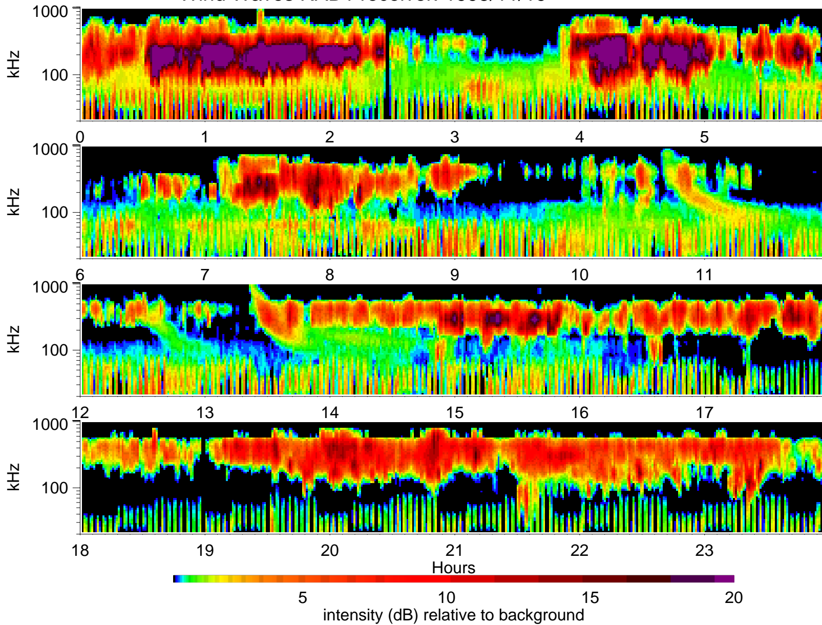
Wind Waves RAD1 receiver: 1995/11/19
