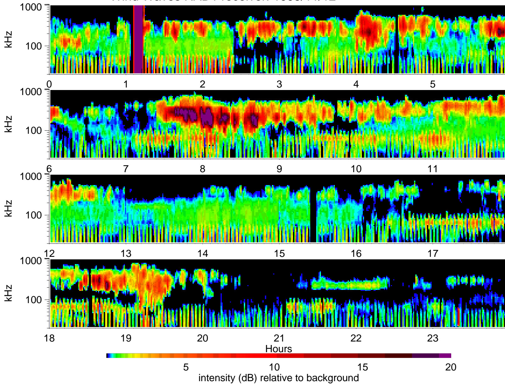
Wind Waves RAD1 receiver: 1995/11/12
