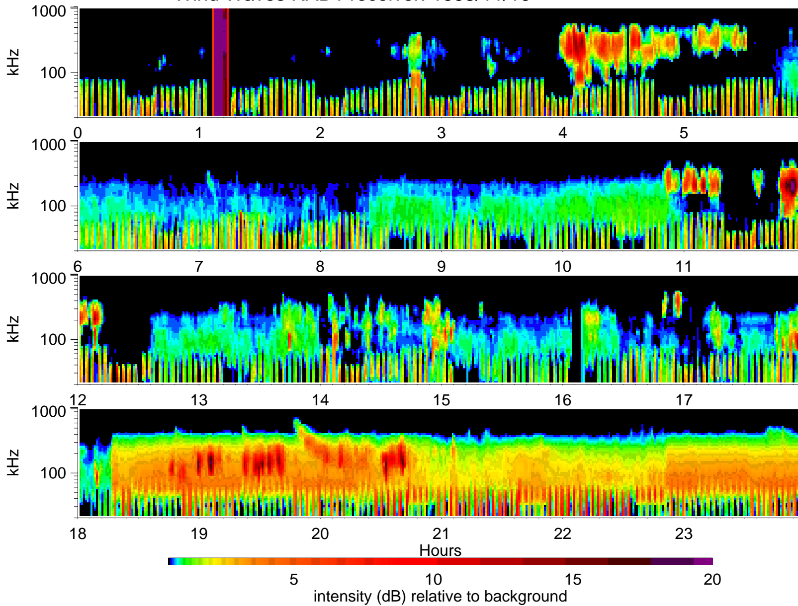
Wind Waves RAD1 receiver: 1995/11/10
