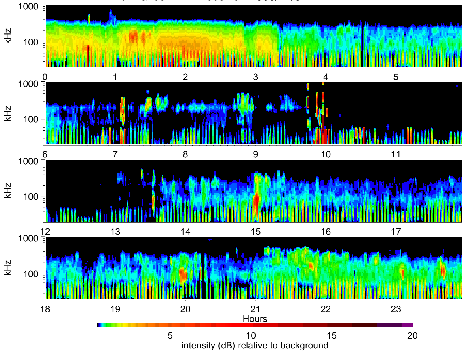
Wind Waves RAD1 receiver: 1995/11/9
