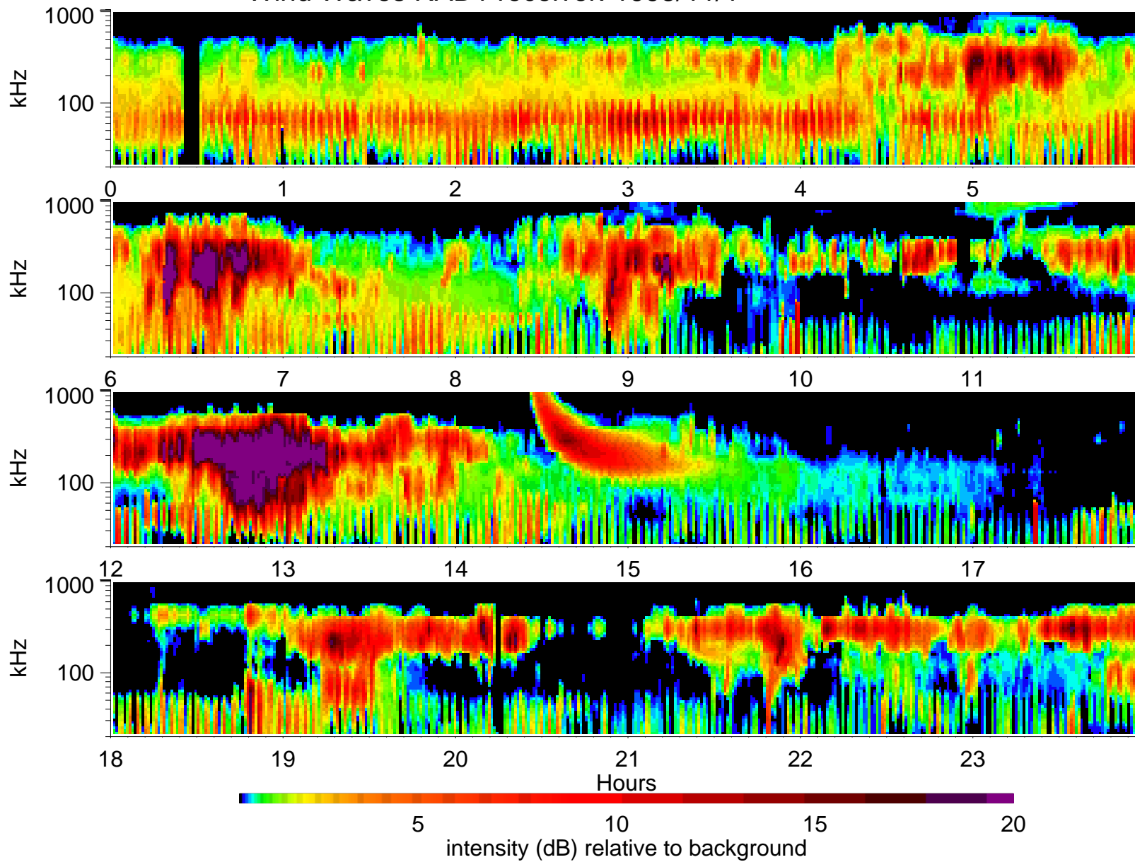
Wind Waves RAD1 receiver: 1995/11/1
