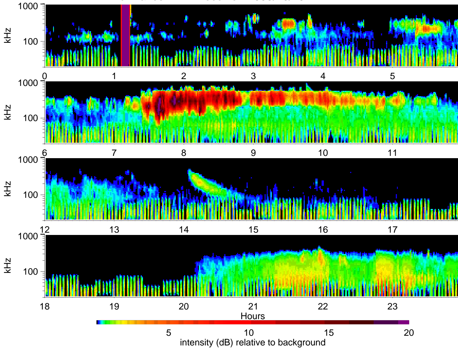
Wind Waves RAD1 receiver: 1995/10/29
