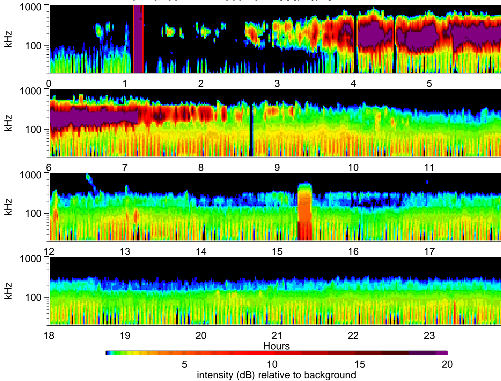
Wind Waves RAD1 receiver: 1995/10/25
