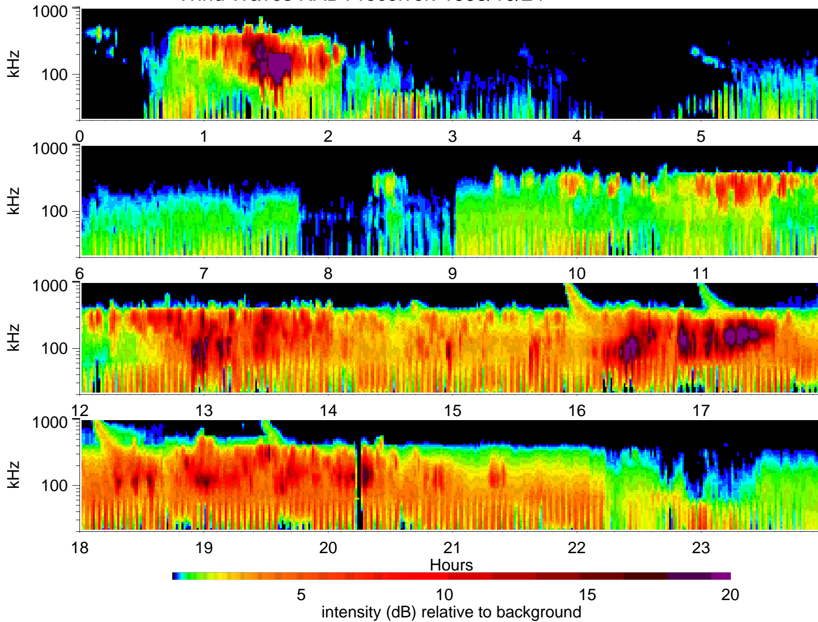
Wind Waves RAD1 receiver: 1995/10/24
