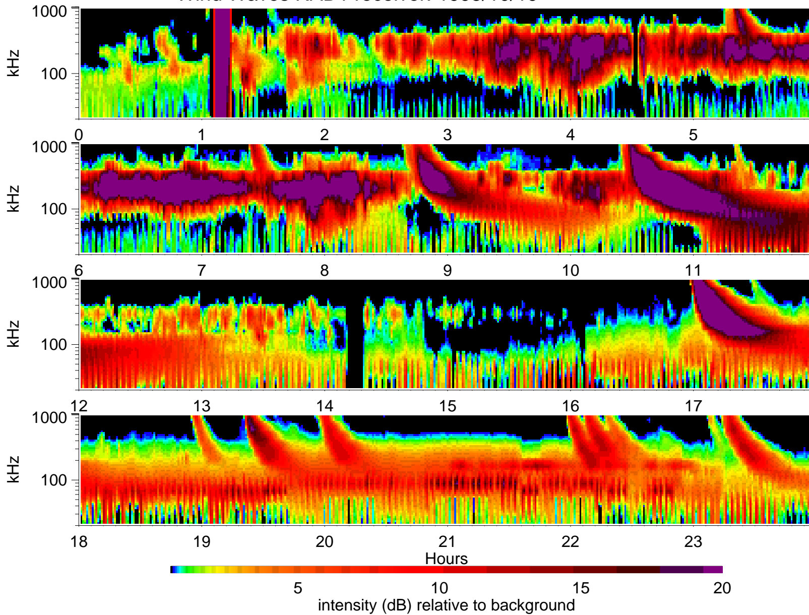
Wind Waves RAD1 receiver: 1995/10/19
