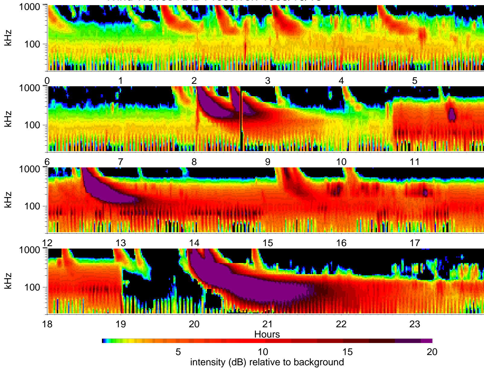
Wind Waves RAD1 receiver: 1995/10/18
