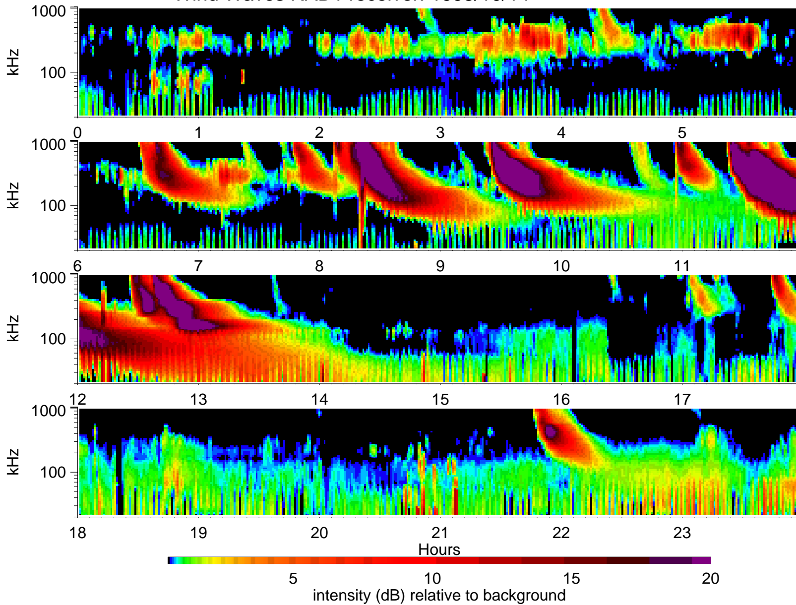
Wind Waves RAD1 receiver: 1995/10/14
