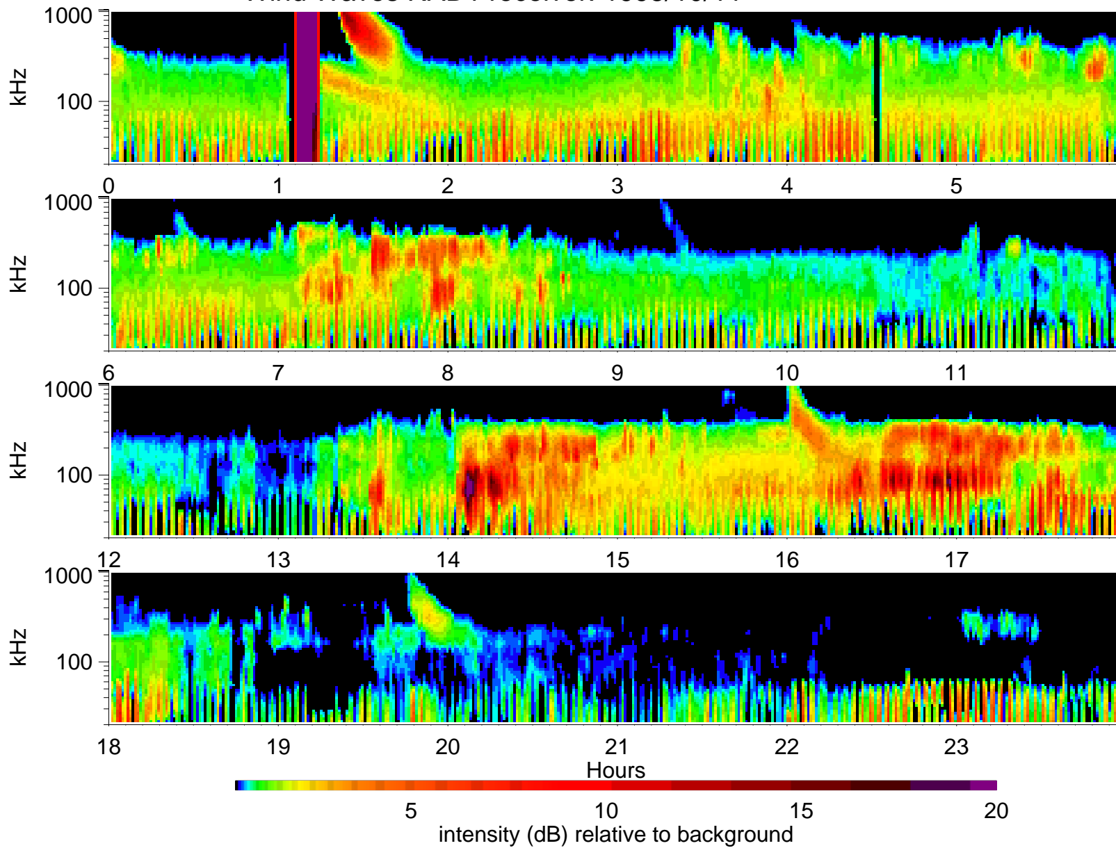
Wind Waves RAD1 receiver: 1995/10/11
