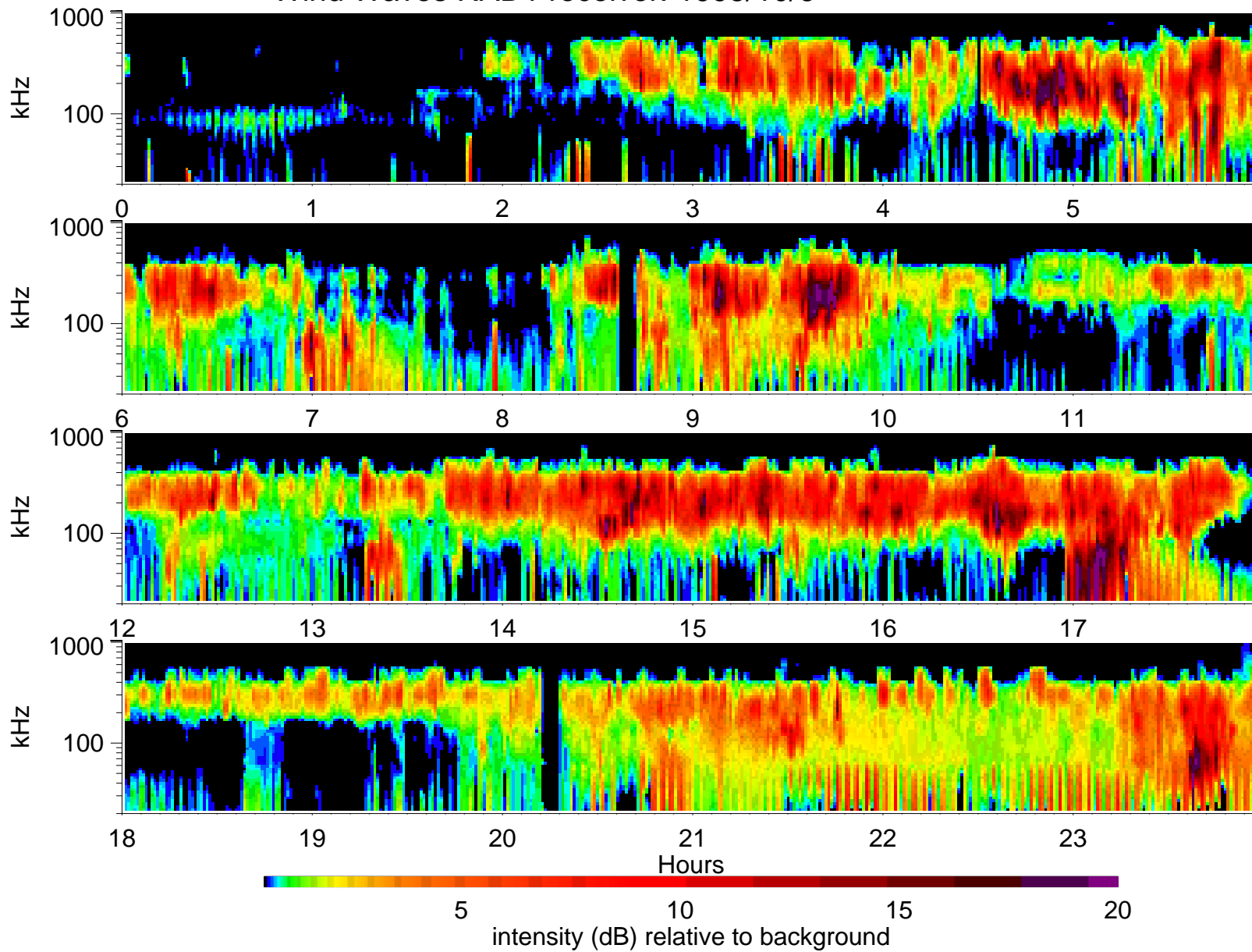
Wind Waves RAD1 receiver: 1995/10/6
