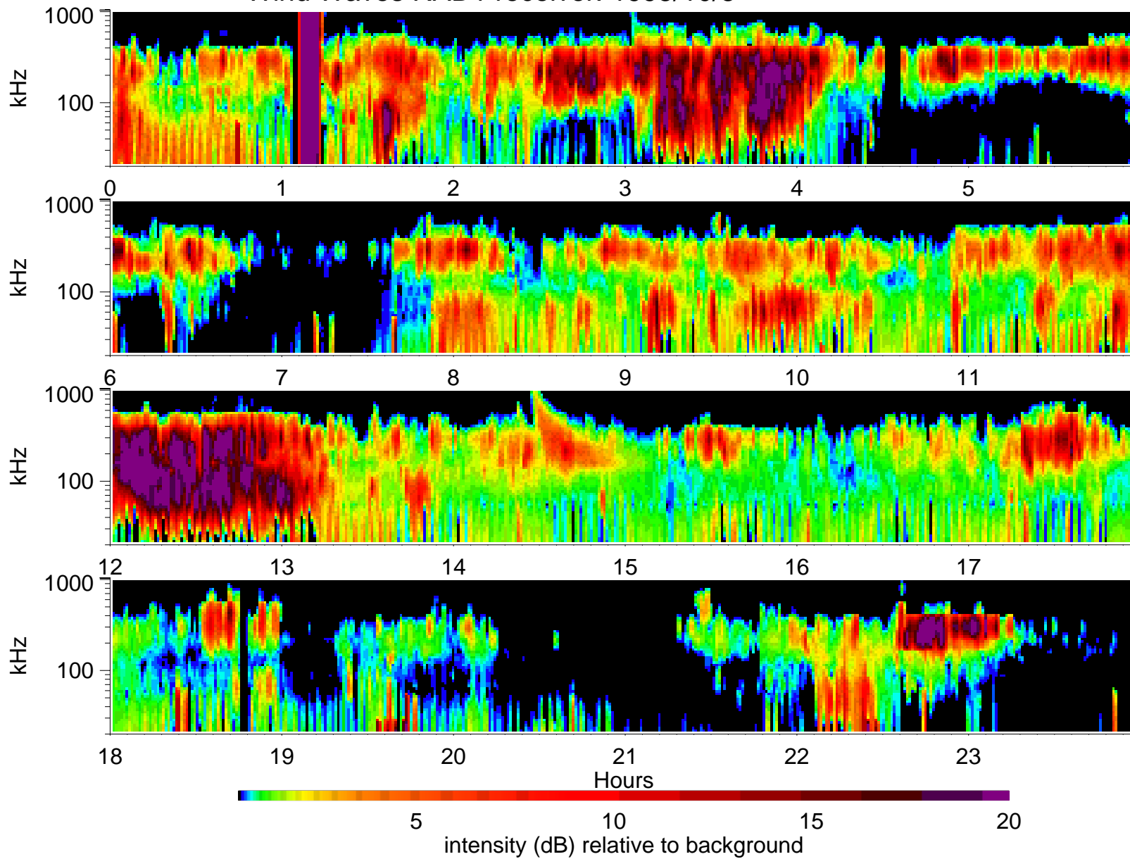
Wind Waves RAD1 receiver: 1995/10/5
