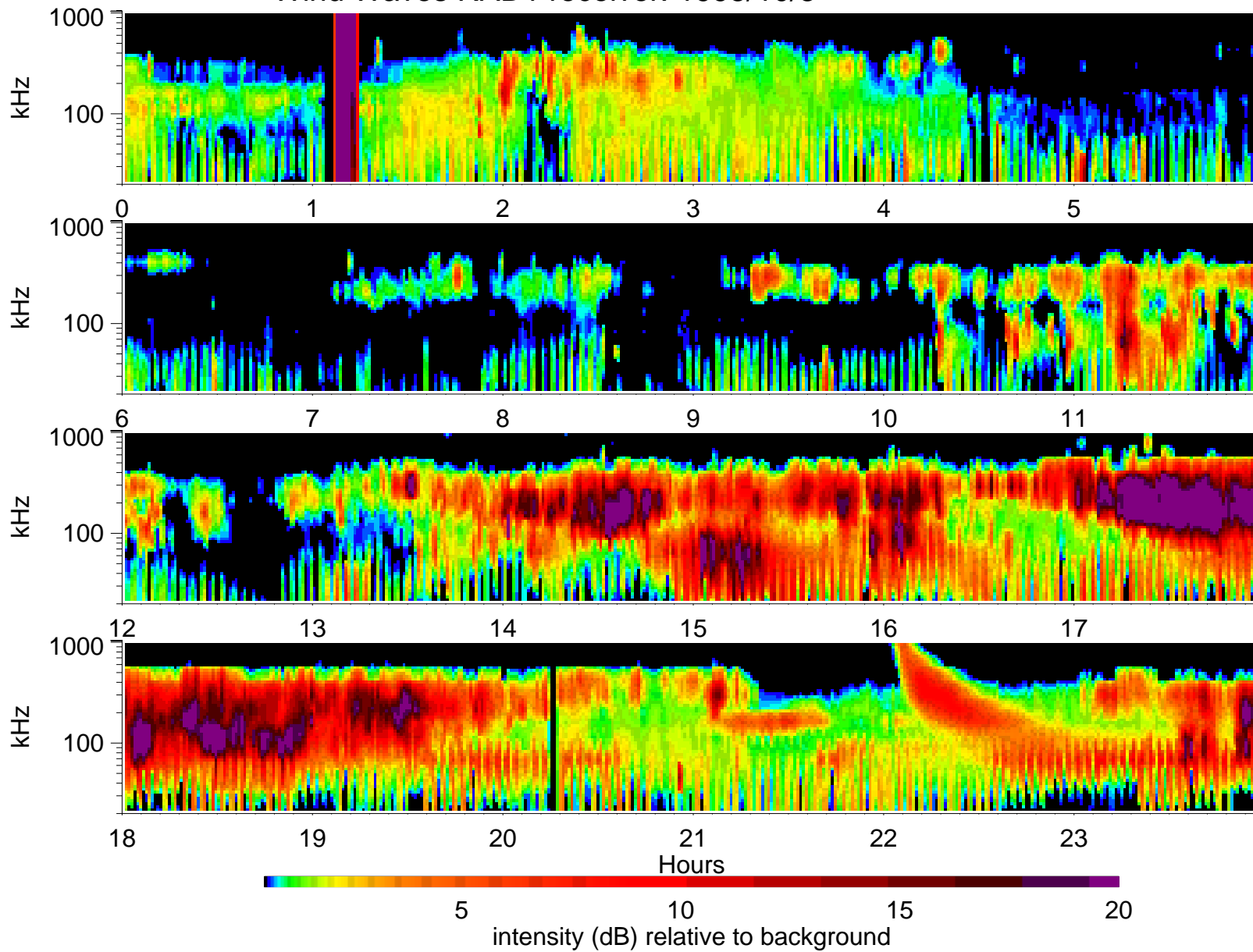
Wind Waves RAD1 receiver: 1995/10/3
