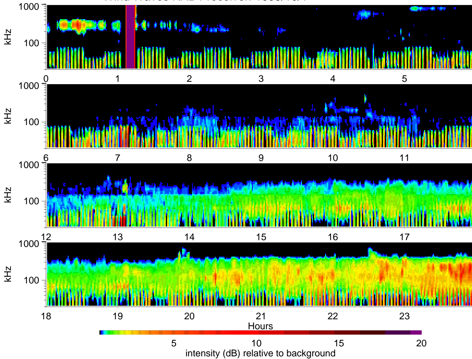
Wind Waves RAD1 receiver: 1995/10/1
