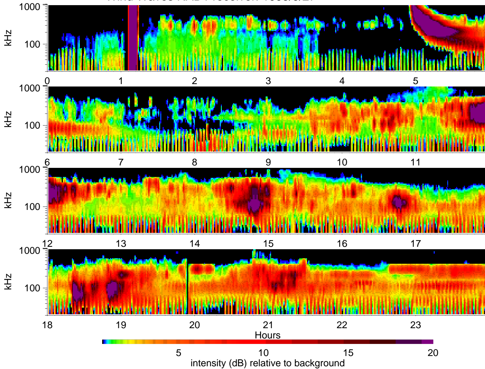
Wind Waves RAD1 receiver: 1995/9/27
