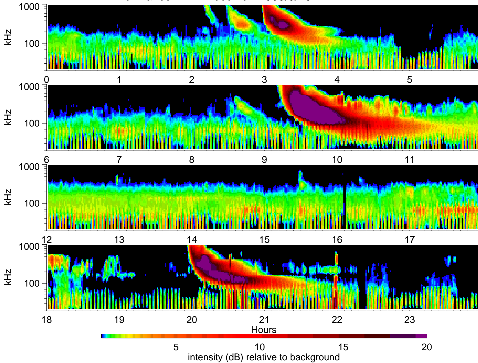
Wind Waves RAD1 receiver: 1995/9/26
